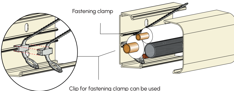
Clip for fastening clamp can be used at any point in the cable duct
