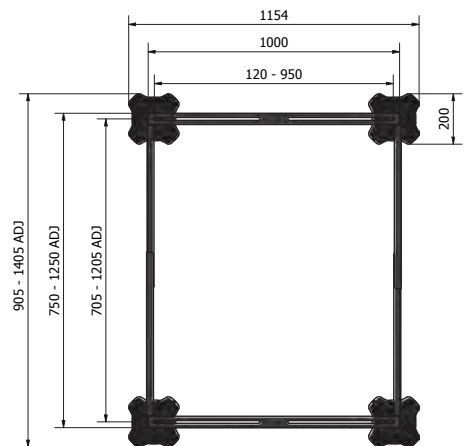
BN8411 Maxi Frame Weight: 16 kg
