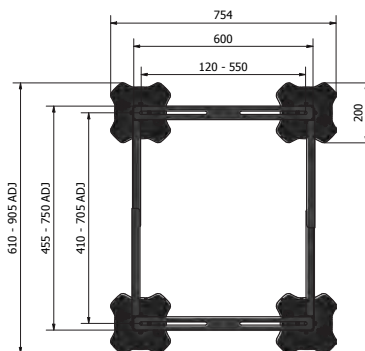
BN8410 Micro frame Weight: 11.5 kg
