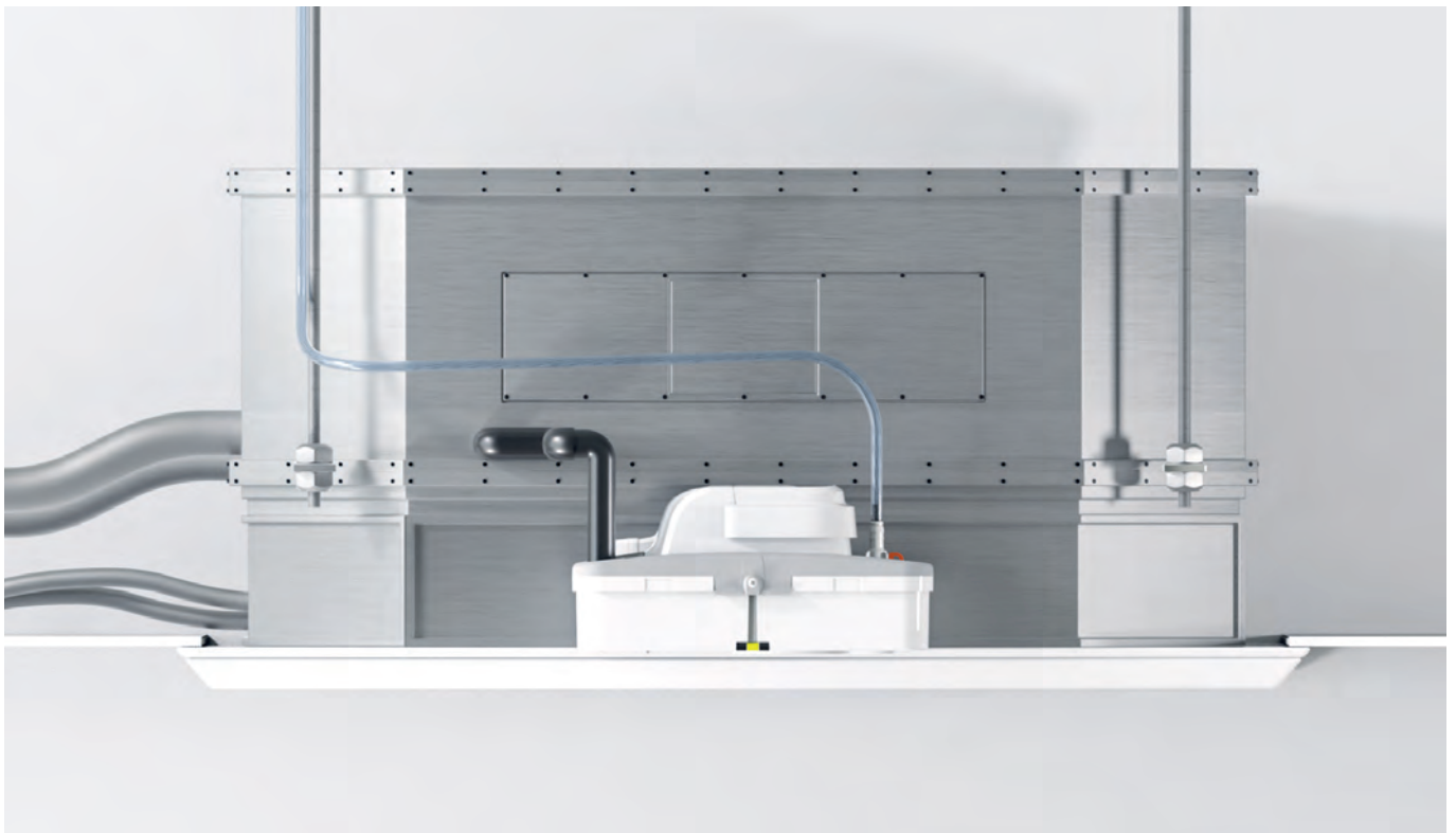
Max Hi-Flow screw mounted to cassette unit
