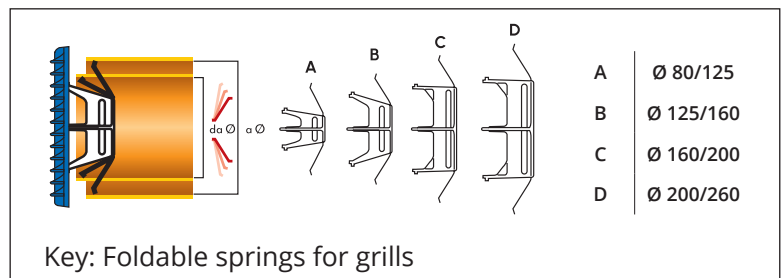
Universal metal grills
