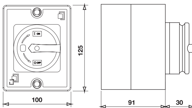
Petit, 20-32 A, 4 pôles
