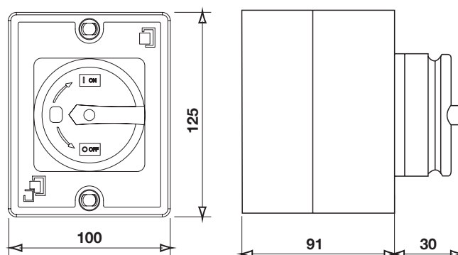
Petit, 20-32 A, 4 pôles
